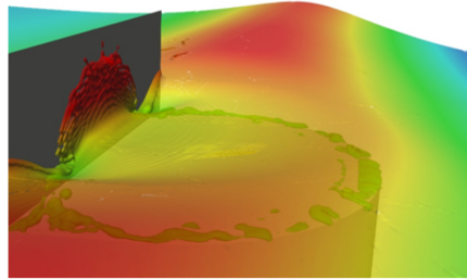
Modelling greenwater over-topping and run-up event at bow of floating structure
